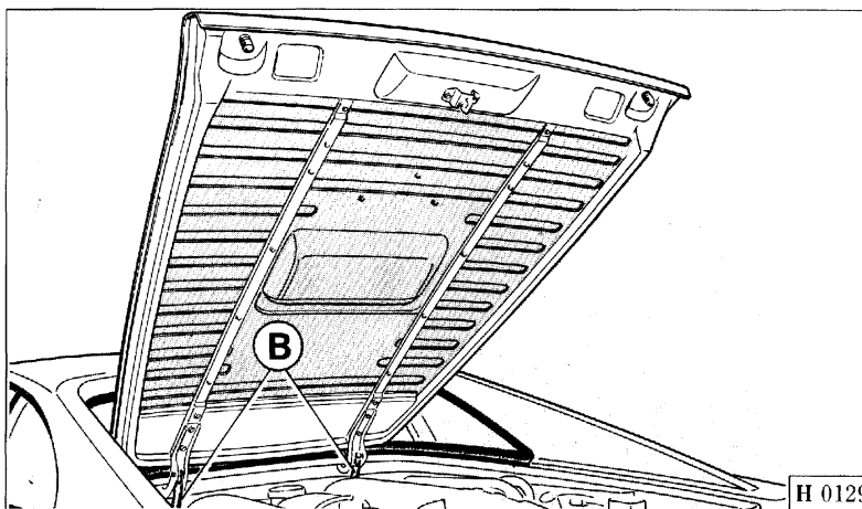
Fig. 33 - Engine cover
