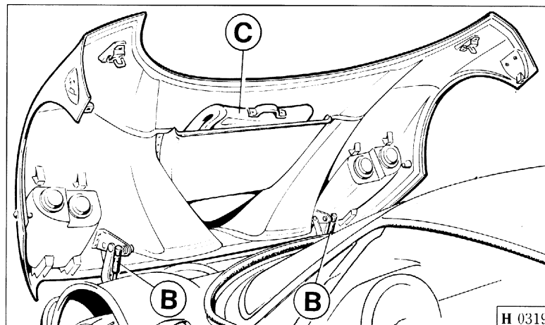
Fig. 21 - Front hood
