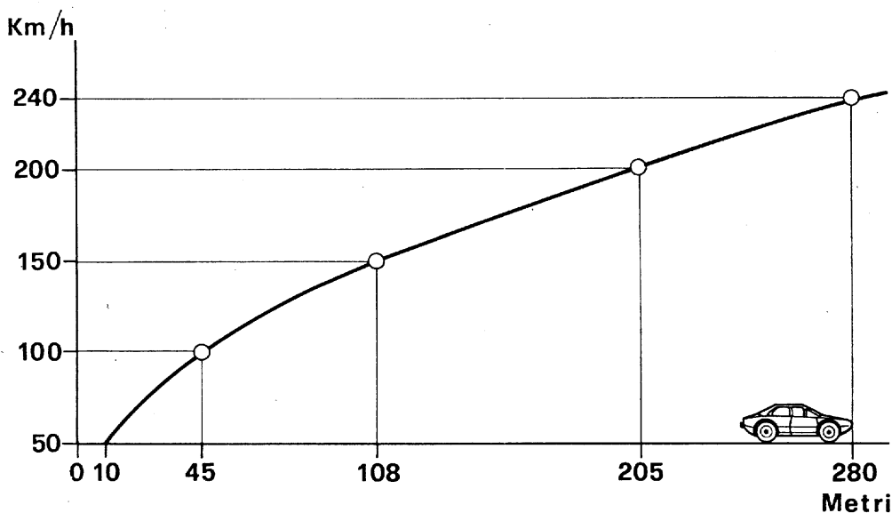
90) Diagram of braking distances.
