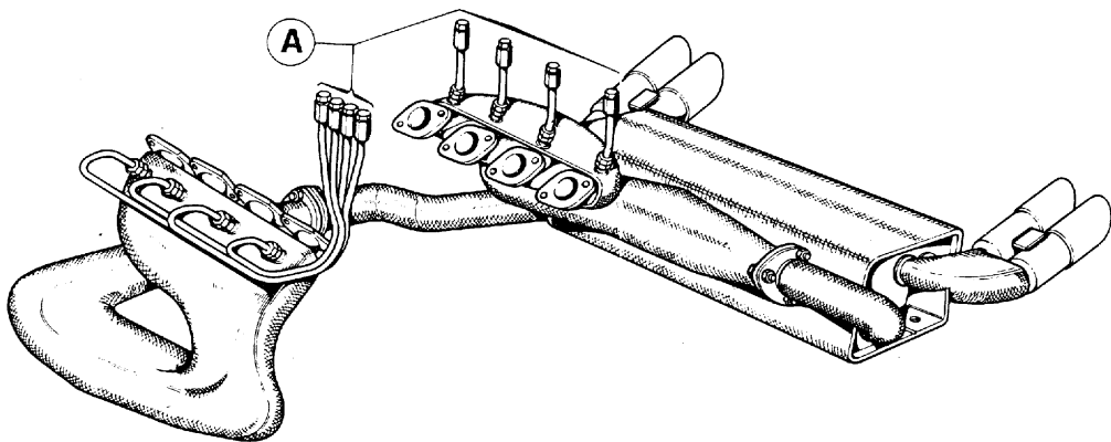
54) Exhaust system with gas analysis probes. A - Gas analysis probes.
