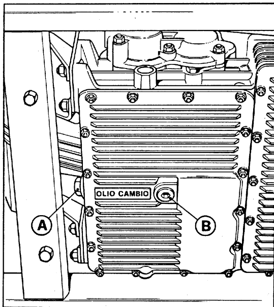
75) Gear-box differential. A - Filler and oil level plug; B - Oil drain plug.
