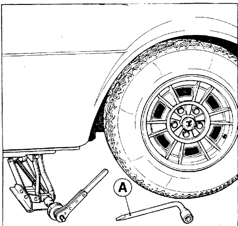
40) Jacking up the rear wheel.
