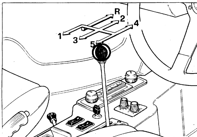
21) Gear lever position.
