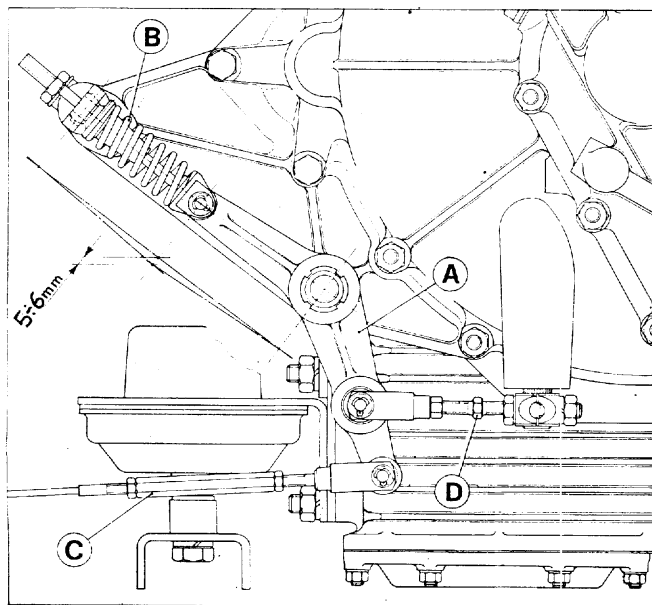
74) Layout of clutch control. A - Lever; B - Helper spring; C-D - Adjustable control rods.
