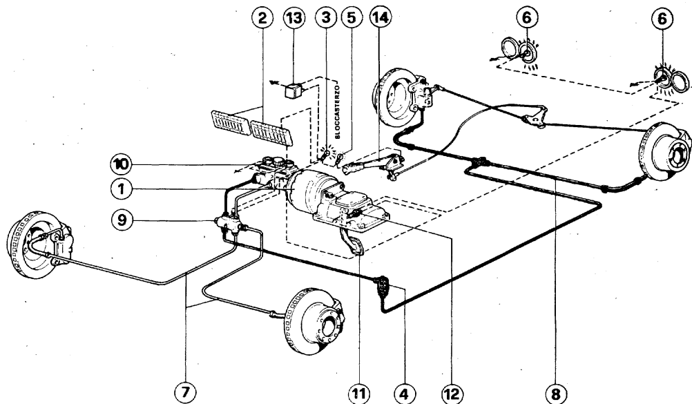
85) Diagram of the braking system.
