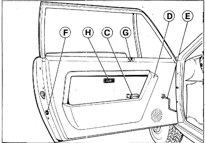
15) Opening from inside.
