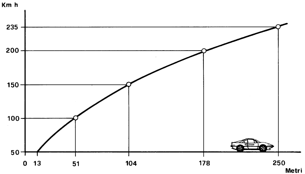
82) Diagram of braking distances.
