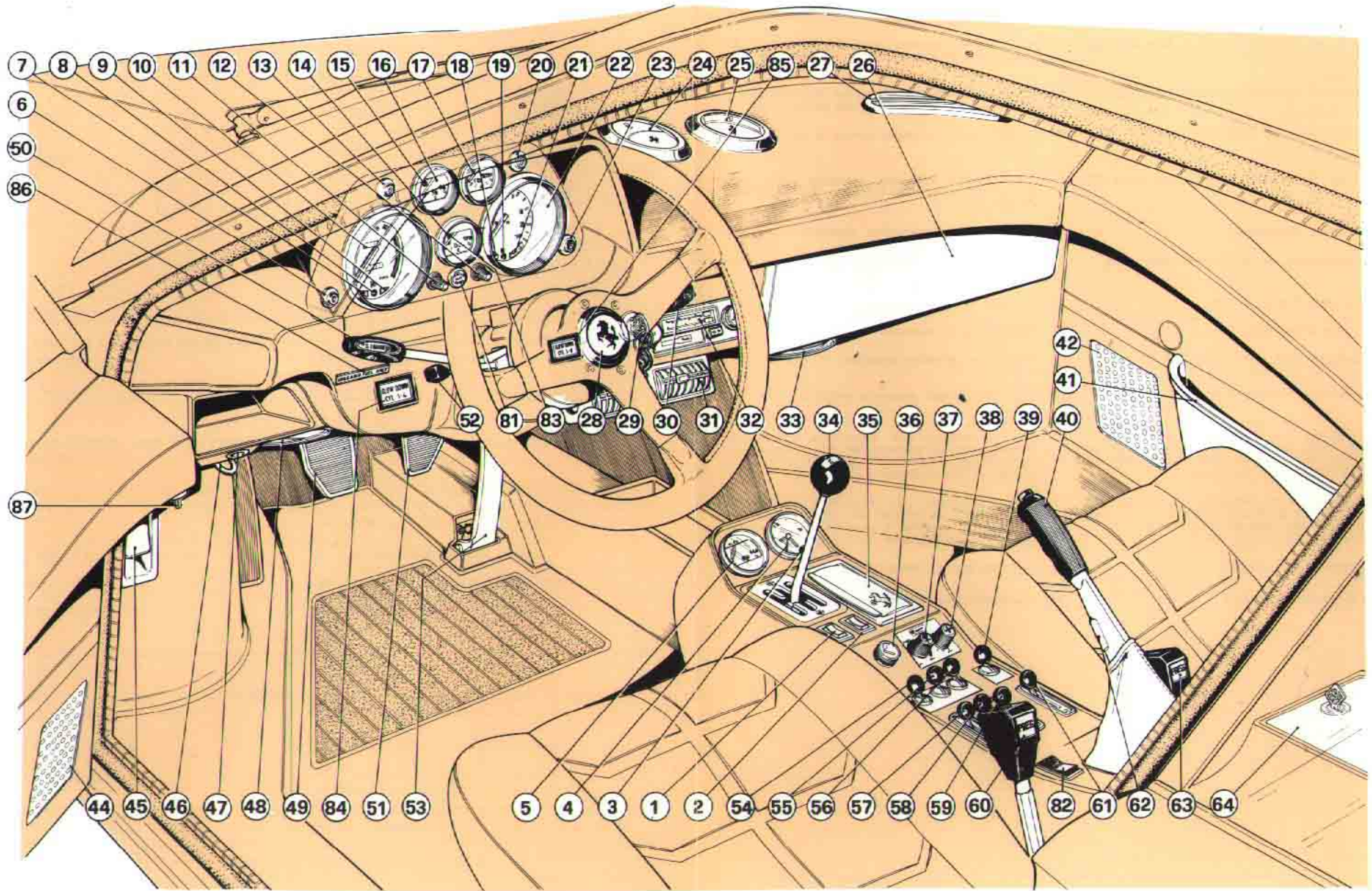
16) Instruments and controls.
