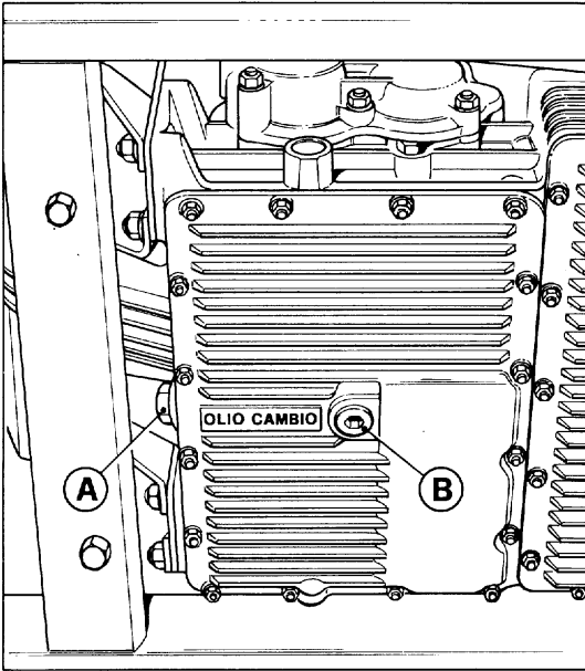
71) Gear-box differential. A - Filler and oil level plug; B - Oil drain plug.
