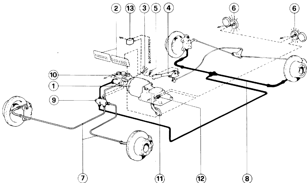
77) Diagram of the braking system.
