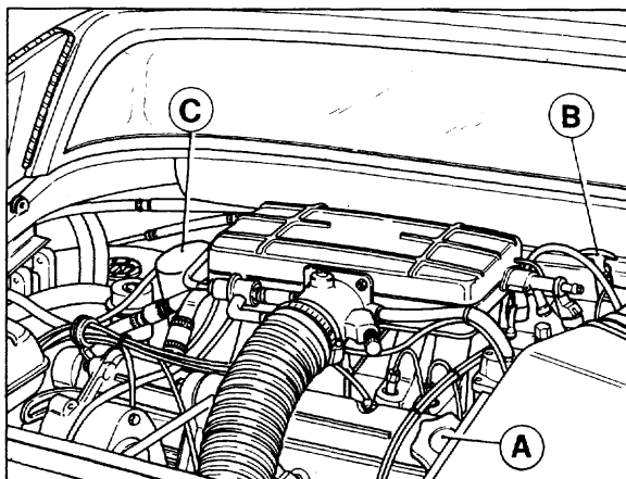
52) Engine lubricant accessories. A - Oil filler cap; B - Dipstick; C - Engine oil filter.
