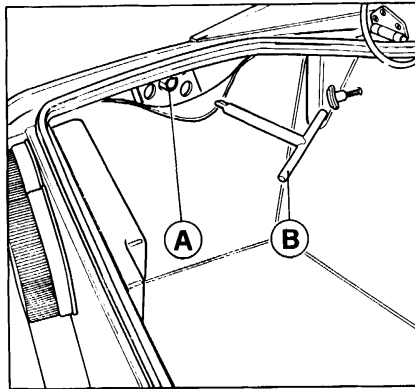
Fig. 41 - Emergency opening
