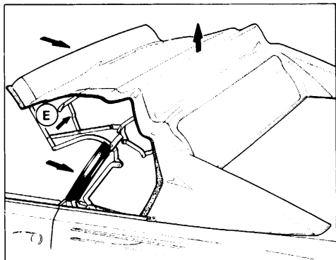
100) - Soft top opening E - Transversal member
