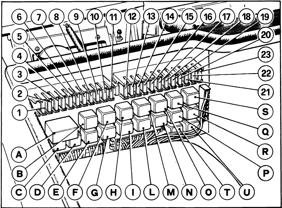
91) Fuses and relays
