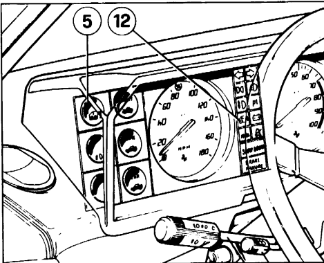
Fig. 93 - Instruments and controls
