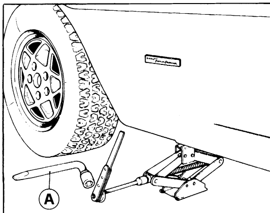
44) Jacking up the rear wheel
