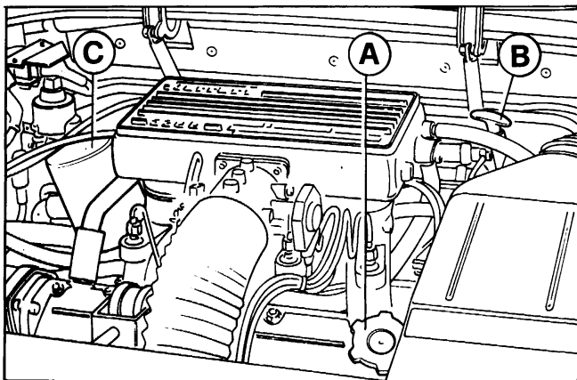
49) Engine lubricant accessories
