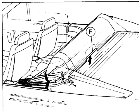
101) Opening the soft top F - Rear cross member
