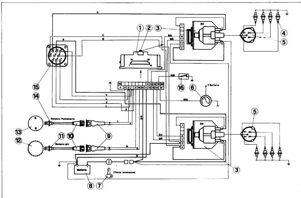
Fig. 59 - Ignition system
